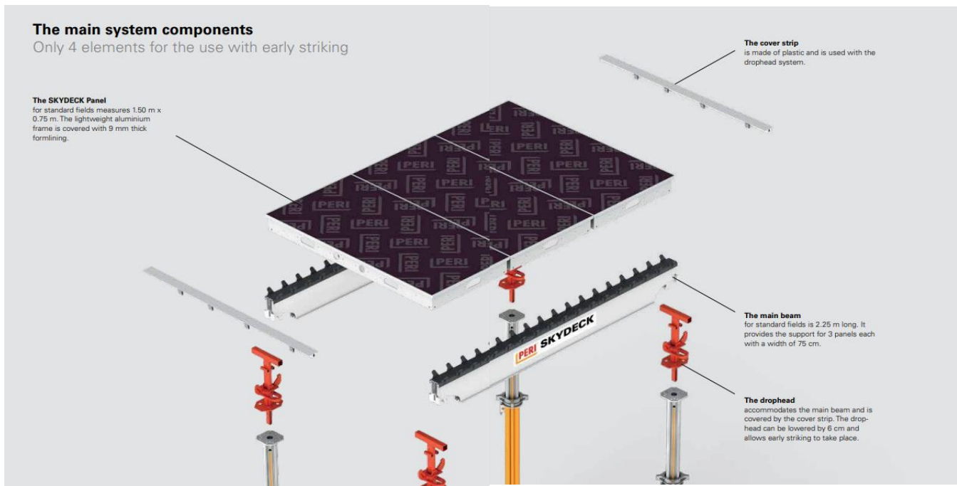
PERI SKYDECK system for concrete floor formwork
